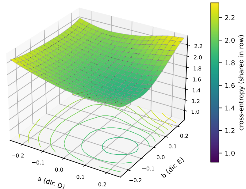
evaluated at r=32 (target) test probe (1,000 imgs), centre CE 1.925
