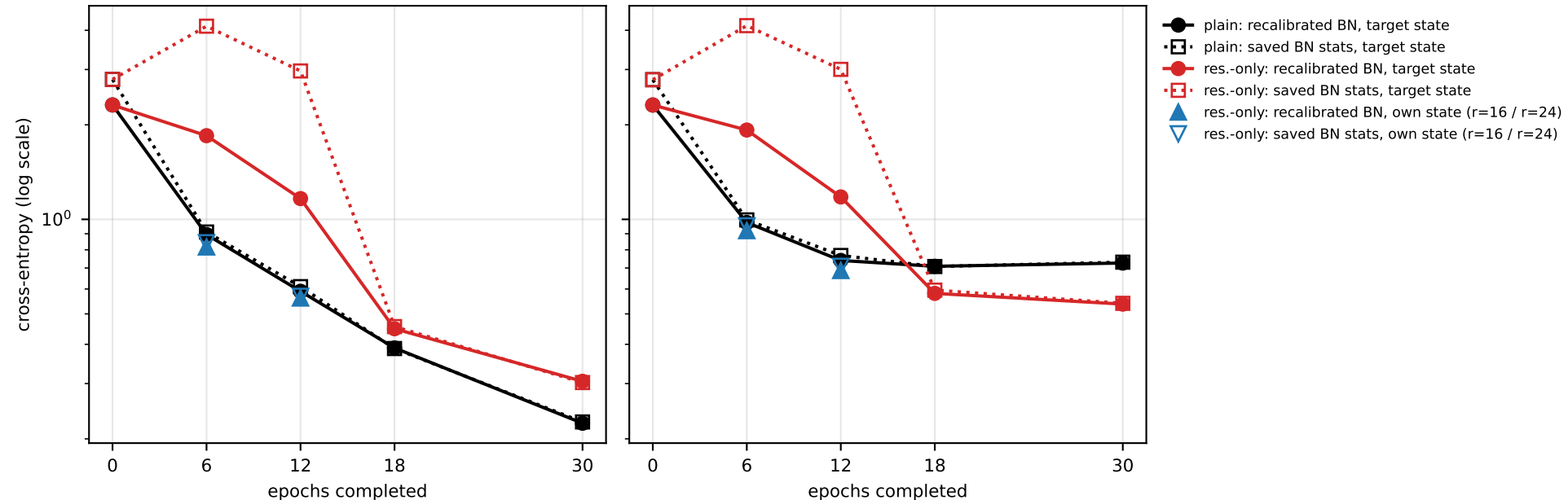
actual checkpoint CE, seed 0, train probe (1,000 imgs)
