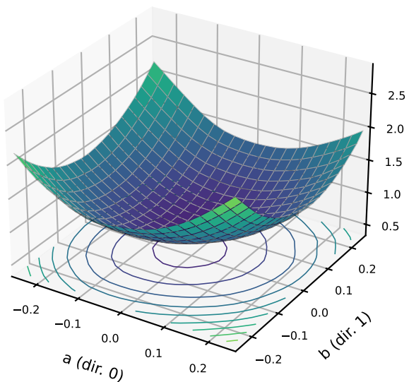
plain, test probe (1,000) centre CE 0.736
