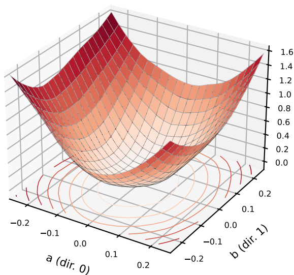
Gaussian-only, test probe (1,000) centre CE 0.568
