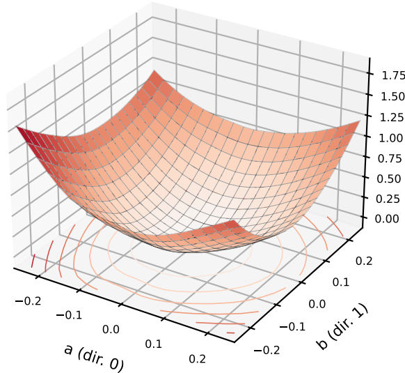
resolution-only, test probe (1,000) centre CE 0.560
