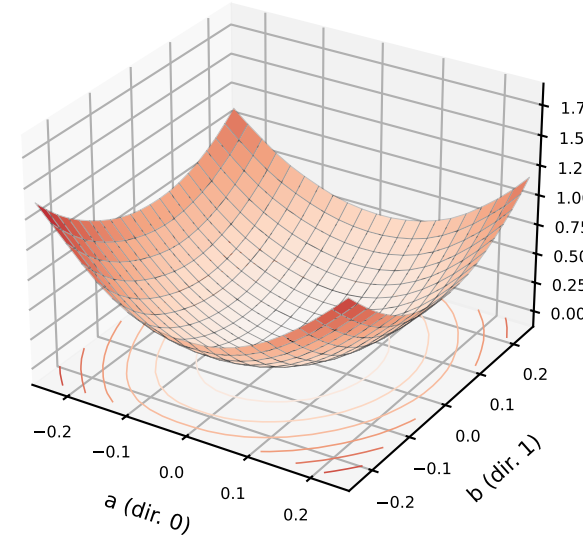
combined, test probe (1,000) centre CE 0.528
