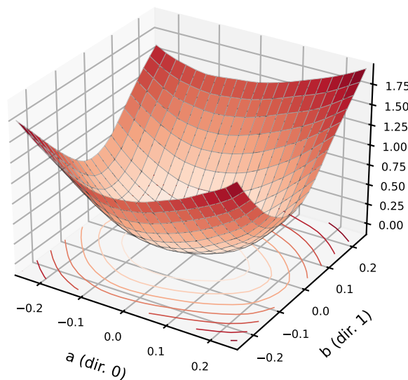
Gaussian-only, test probe (1,000) centre CE 0.569
