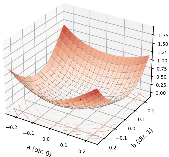
resolution-only, test probe (1,000) centre CE 0.563
