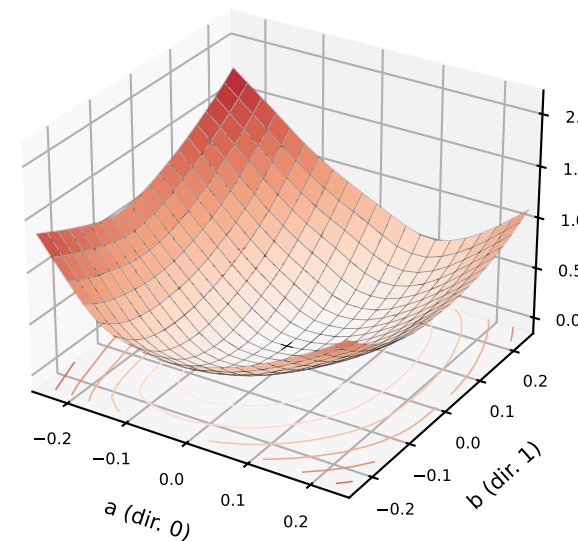
combined, test probe (1,000) centre CE 0.537
