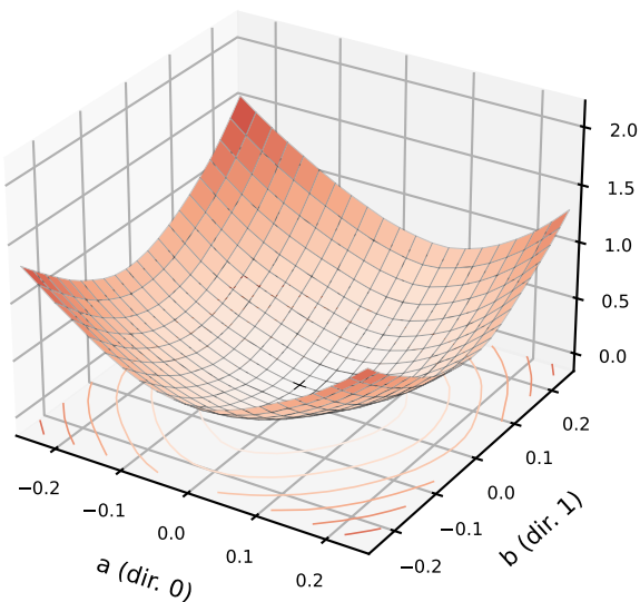
plain, test probe (1,000) centre CE 0.761
