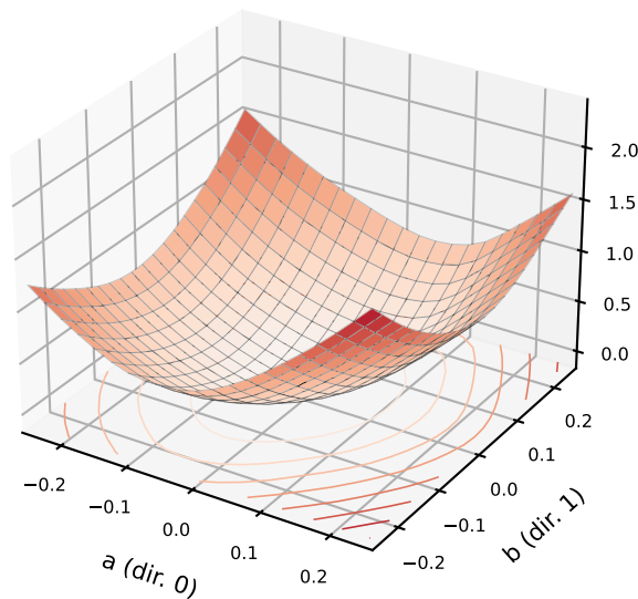
resolution-only, test probe (1,000) centre CE 0.573
