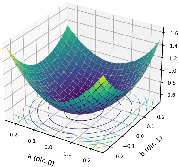
state after {'resolution': 32, 'sigma': 0.0} test probe (1,000), centre CE 0.545
