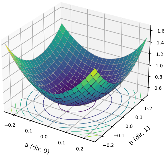
state before {'resolution': 32, 'sigma': 0.3} test probe (1,000), centre CE 0.543
