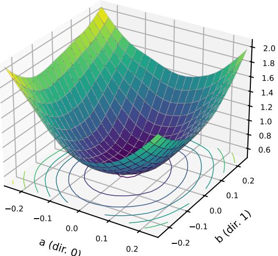
state before {'resolution': None, 'sigma': 0.3} test probe (1,000), centre CE 0.578
