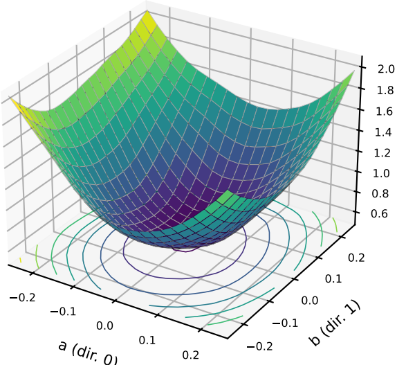
state after {'resolution': None, 'sigma': 0.0} test probe (1,000), centre CE 0.582
