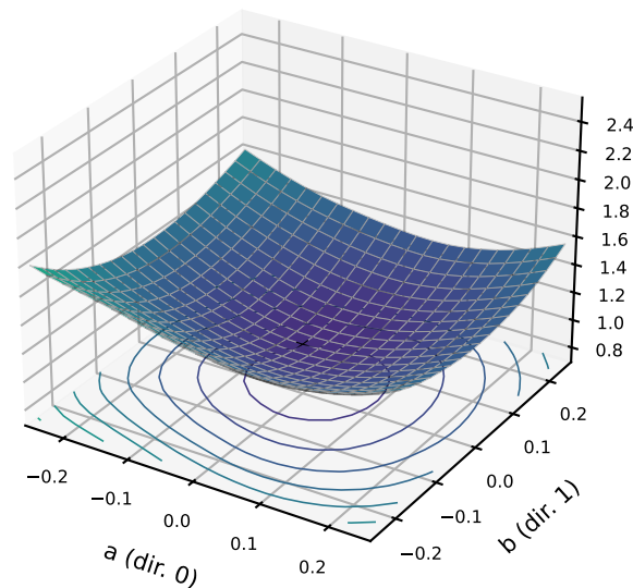
state after {'resolution': 24, 'sigma': None} test probe (1,000), centre CE 1.060
