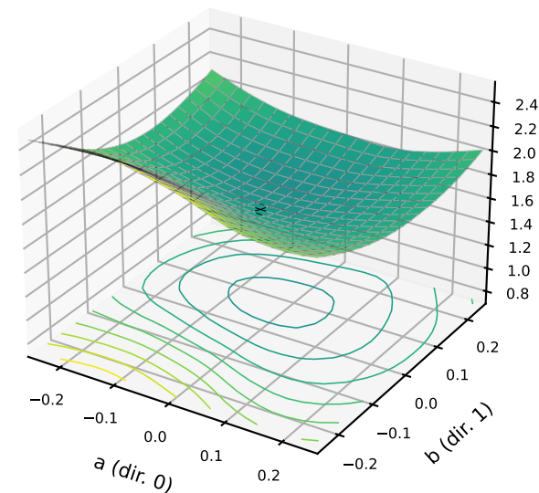
state r=32 {'resolution': 32, 'sigma': None} test probe (1,000), centre CE 1.768
