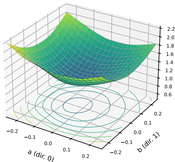
state after {'resolution': 32, 'sigma': None} test probe (1,000), centre CE 1.209
