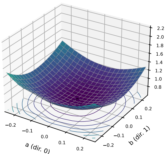
state before {'resolution': 24, 'sigma': None} test probe (1,000), centre CE 0.693
