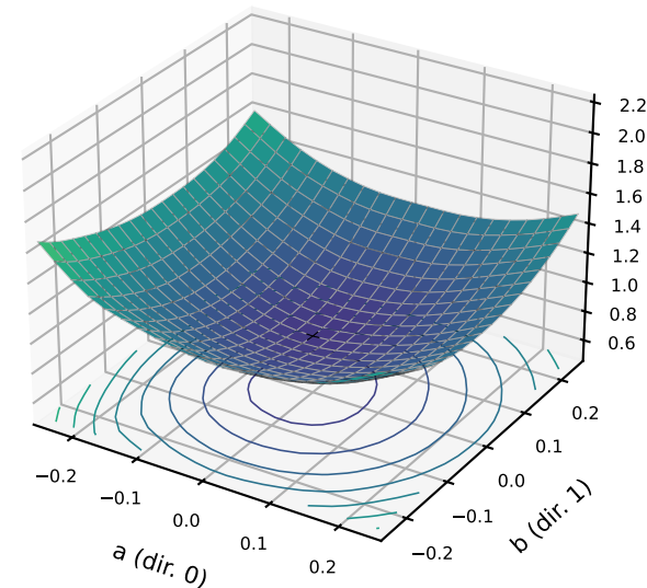
state r=16 {'resolution': 16, 'sigma': None} test probe (1,000), centre CE 0.916
