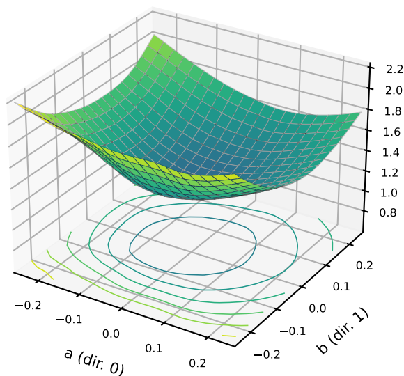
state after {'resolution': 32, 'sigma': None} test probe (1,000), centre CE 1.209
