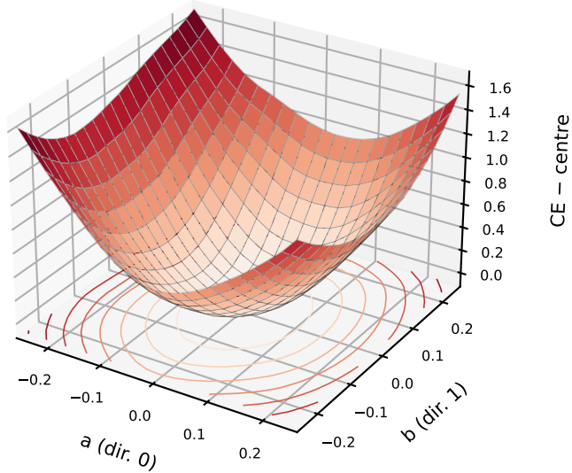
state before {'resolution': None, 'sigma': 0.3} test probe (1,000), centre CE 0.578
