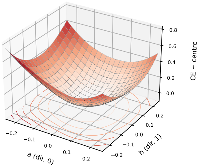
state before {'resolution': 16, 'sigma': None} test probe (1,000), centre CE 0.924
