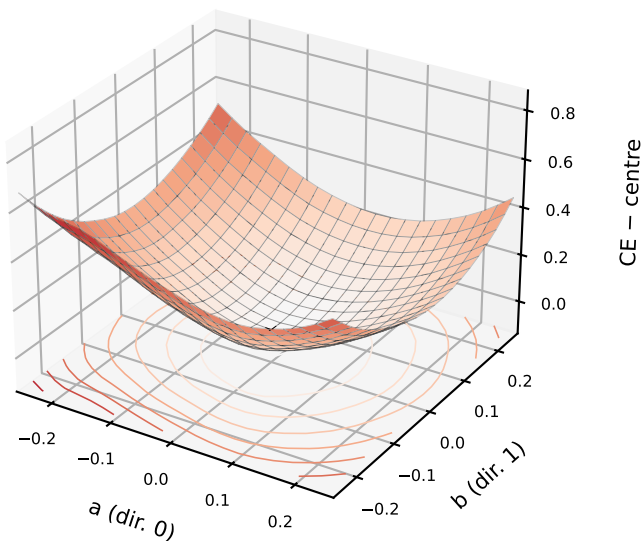
state before {'resolution': 16, 'sigma': None} test probe (1,000), centre CE 0.924
