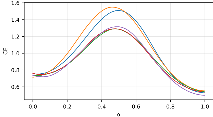
resolution-only ( \alpha=0 ) \rightarrow combined ( \alpha=1 ), test probe (1,000)
