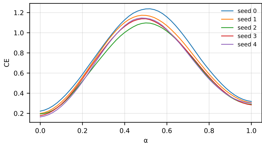
plain ( \alpha=0 ) \rightarrow Gaussian-only ( \alpha=1 ), train probe (1,000)
