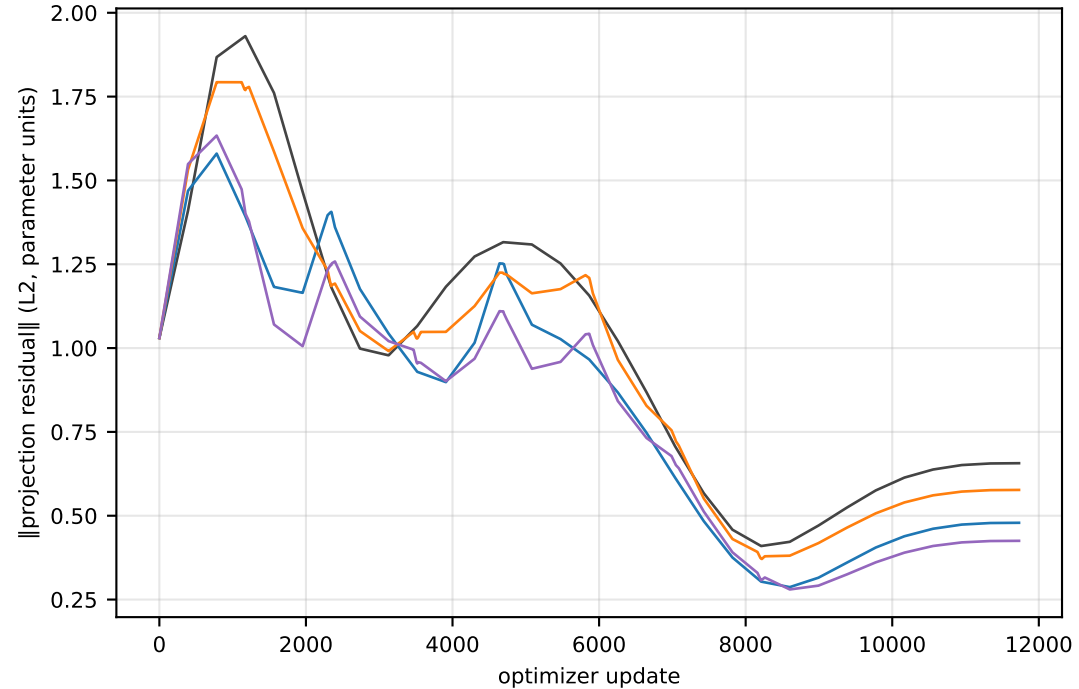
residual after projecting on 10 components (seed 3)
