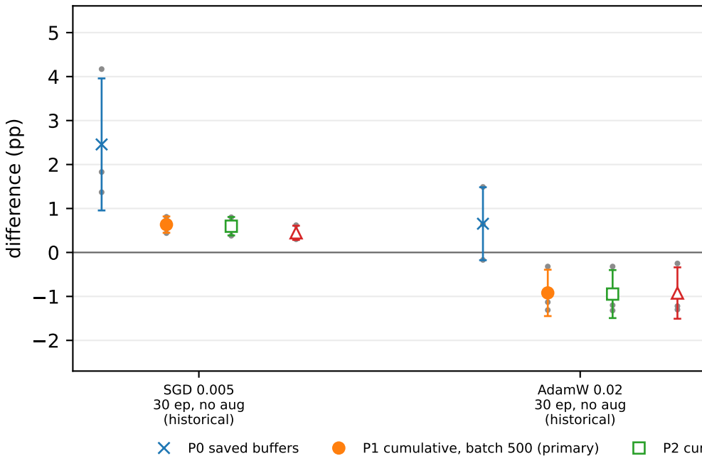
R - SDPoint, test accuracy (pp, seed-paired)
