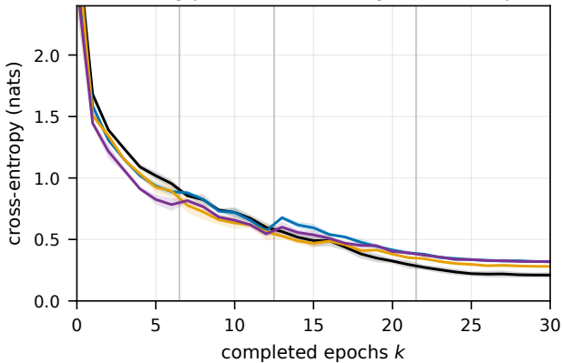
(c) Training-probe CE (500 images), current path
