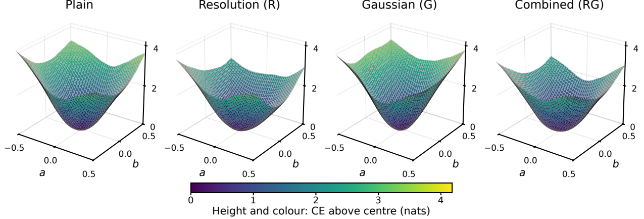
Figure 2: Illustrative loss slices for the four final seed-0 models: CIFAR-10 / ResNet-20-BN / SGD, 30 epochs, 1k-image training probe, pointwise BatchNorm recalibration. Surfaces join the 41-by-41 measured values of L(\theta_0 + ad_1 + bd_2) - L(\theta_0) . Viewing angles, axis limits and colour scales are identical. Directions share random draws but use each model’s filter norms. These slices illustrate relative perturbations in one seed, not a general ordering of curvature.
