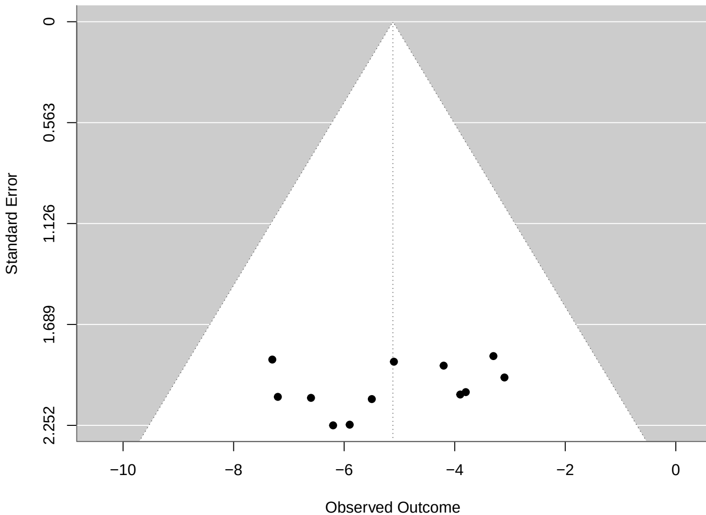
Funnel plot: Systolic blood pressure at 12 weeks
