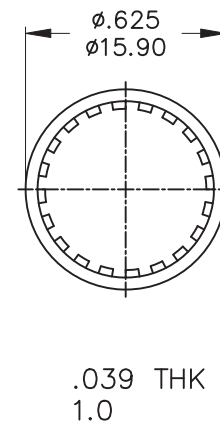
LOCK WASHER
