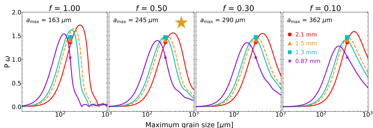
Figure 5.11: Curves of P\omega multiplied by best-fit SF (Equation ??) to compare to \mathcal{P}_{F,\text{obs}} . Markers are \mathcal{P}_{F,\text{obs}} , listed in Table ?. The best-fit (lowest \chi^2 , Equation ??) is represented with a gold star. The specific results of the fit can be found in Table ?. Wavelengths that are not included in the fit for the SF have a dashed line. Q: Q1: Make markers just the outline if not in the fit? Or just a dashed line, okay? Q2: Should I make the x-axes different? As in, at lower f values, should I start at a higher x_{\text{min}} and go to a higher x_{\text{max}} so you can see the entire curve better?
