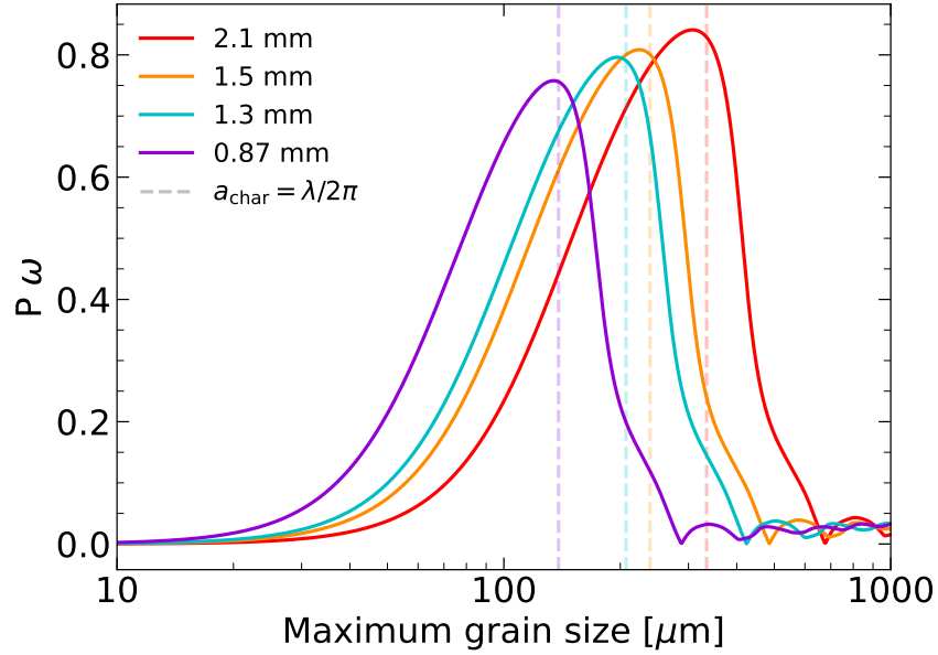
Figure 5.10: Polarization curves ( P_\omega ) versus grain size for each wavelength. Over-plotted as a dashed line with matching colour is the characteristic grain size. Locations of maximum P_\omega and characteristic grain size are listed in Table ???. This is a recreation of Figure 4 from ?
