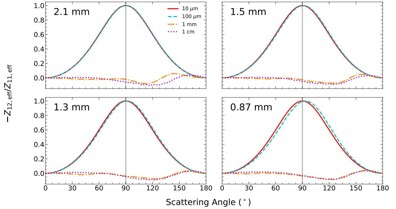
Figure 5.8: Degree of polarization as a function of scattering angle for maximum grain sizes of 10\ \mu\text{m} , 100\ \mu\text{m} , 1\ \text{mm} and 1\ \text{cm} . This is a replication of Figure 2 from ?.
