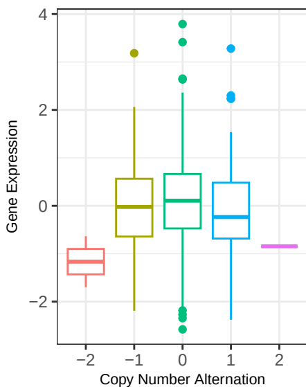
M0.2 CNA v. GE ( r = 0.0034 )
