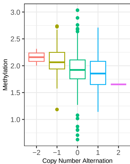
M0.2 CNA v. Methylation ( r = -0.2071 )
