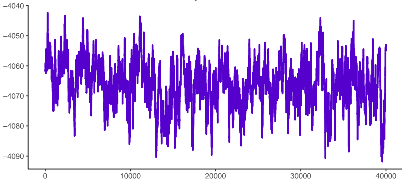
log likelihood
