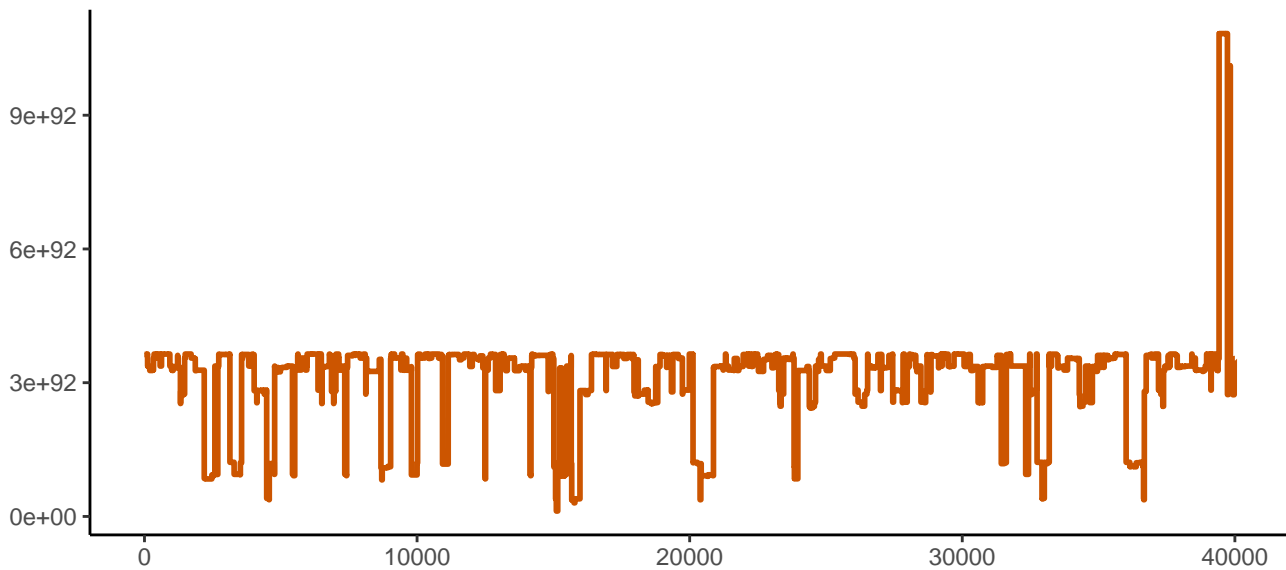
decimal number
