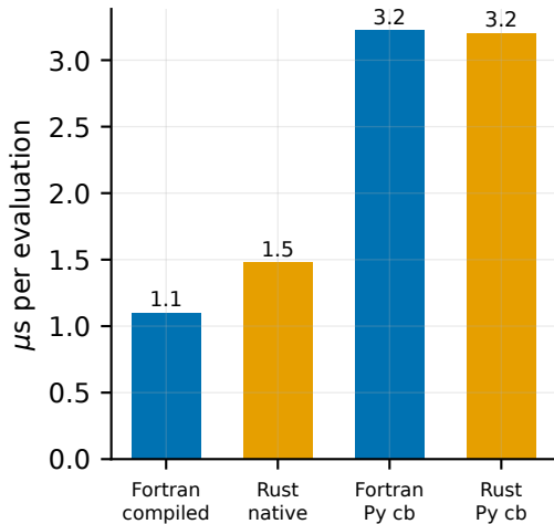
MIG2 call overhead ( n = 10 )
