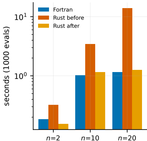
BAYES1 translation repair
