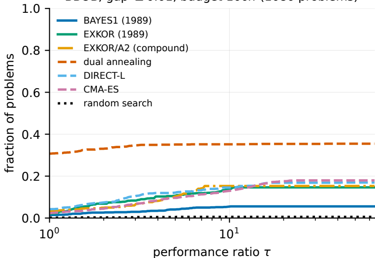
BBOB, gap \leq 0.01 , budget 100n (1080 problems)
