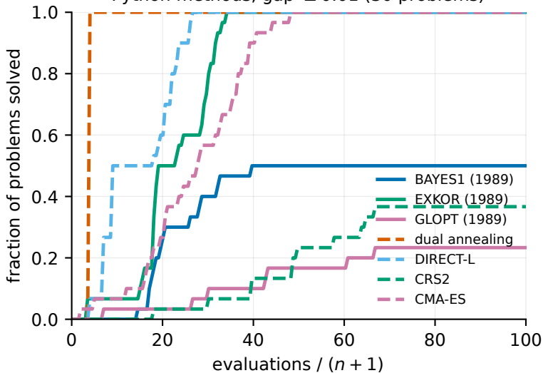
Python methods, gap \leq 0.01 (30 problems)
