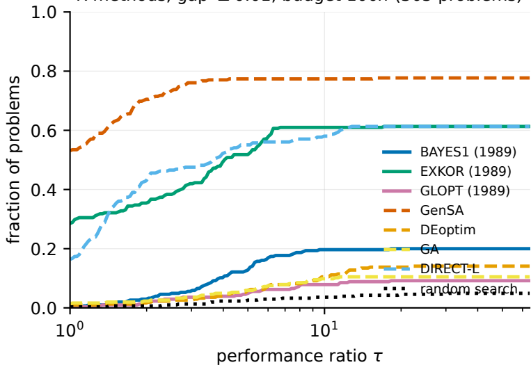
R methods, gap \leq 0.01 , budget 100n (305 problems)
