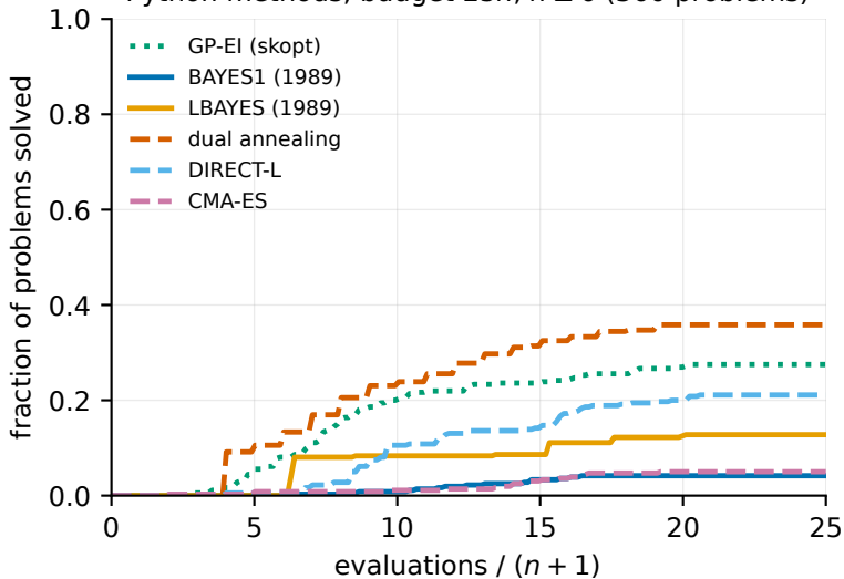
Python methods, budget 25n , n \leq 6 (360 problems)
