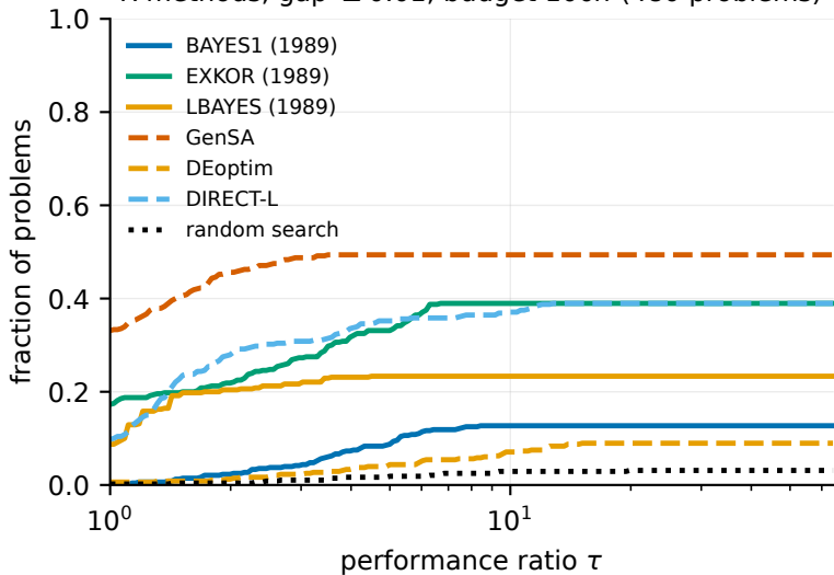
R methods, gap \leq 0.01 , budget 100n (480 problems)
