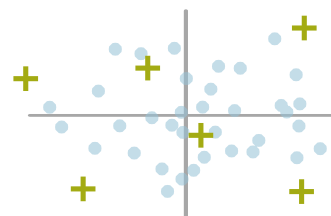
Biplot
