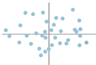
Scatter plot
