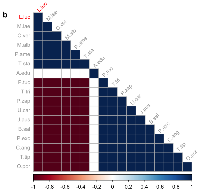
Supplementary Figure 2. 12: Residual between-species correlation from the concurrent ordination (after accounting for the canonical coefficients).
