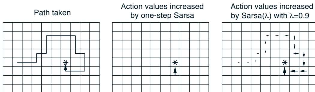
Figure 7.13: Gridworld example of the speedup of policy learning due to the use of eligibility traces.
