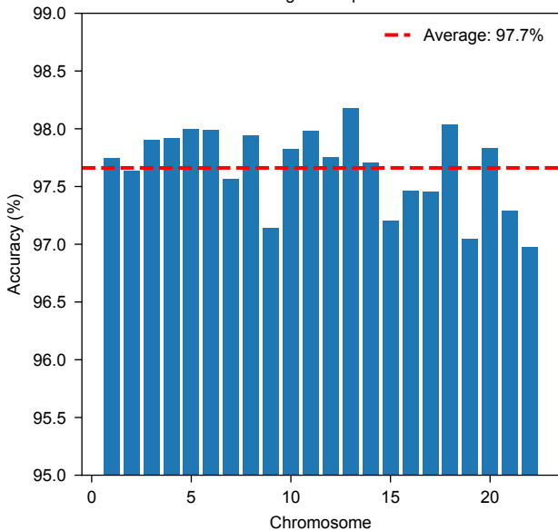
Whole-genome pretrain
