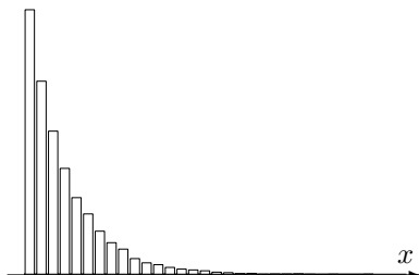
(b) Exponential
