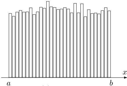
(a) Uniform
