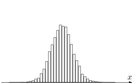
(c) Normal
