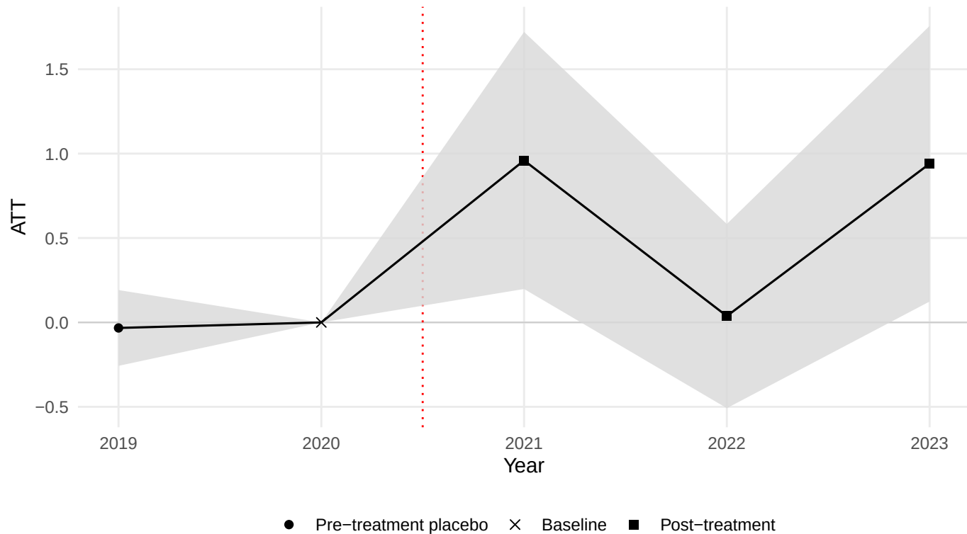
PanelMatch dynamic estimates – cert_tot (CBPS.weight)
