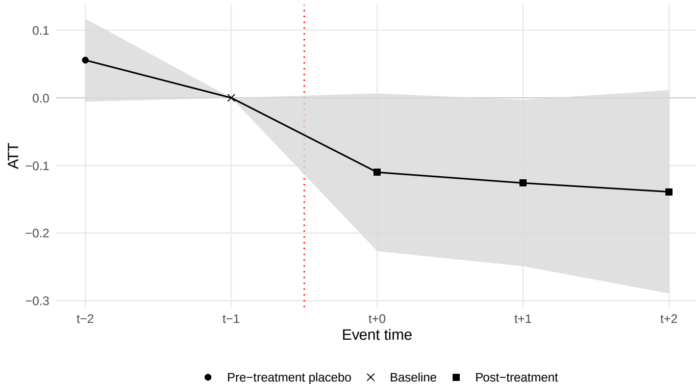
PanelMatch dynamic estimates – n_manodopera (CBPS.weight)
