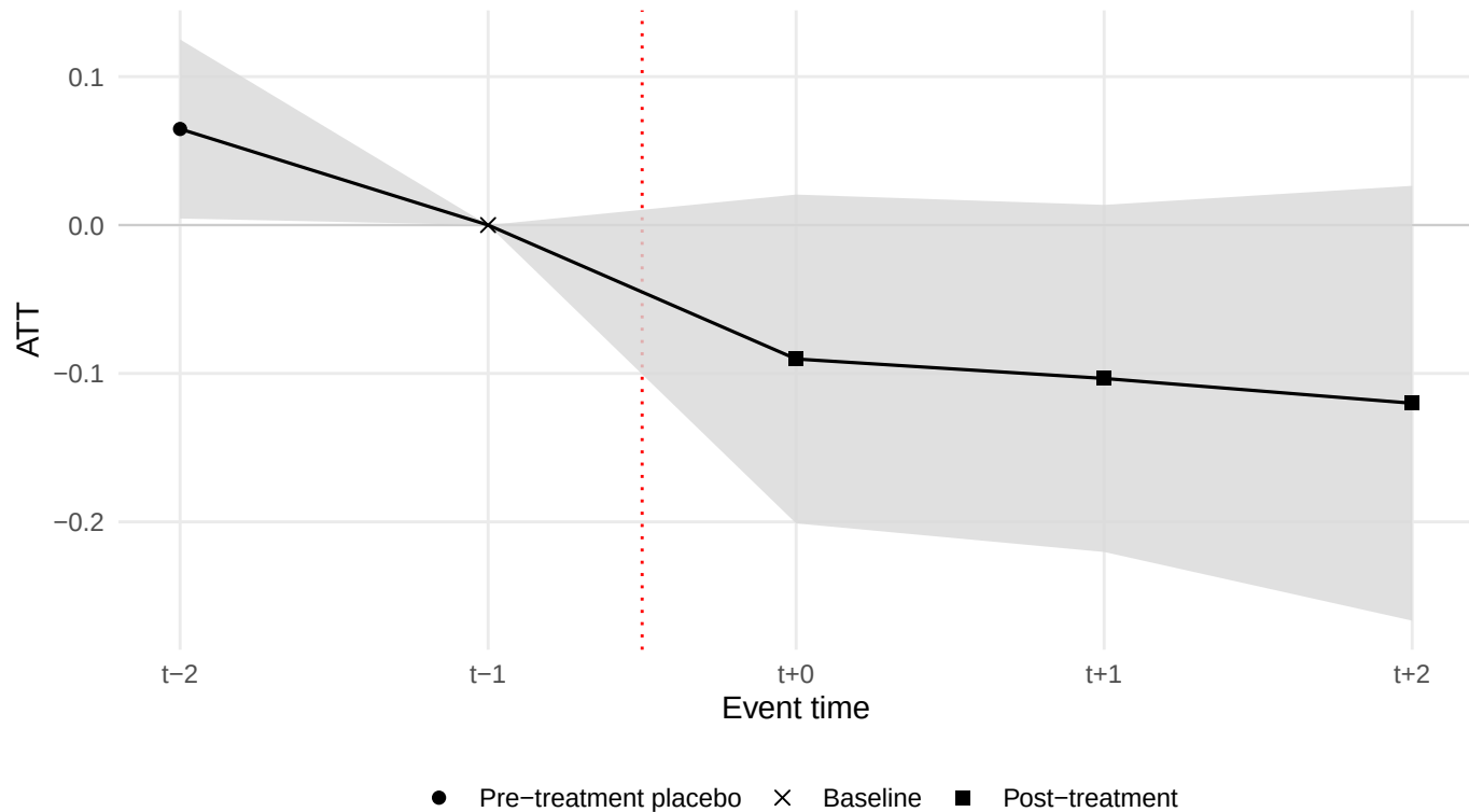
PanelMatch dynamic estimates – n_manodopera_w (CBPS.weight)
