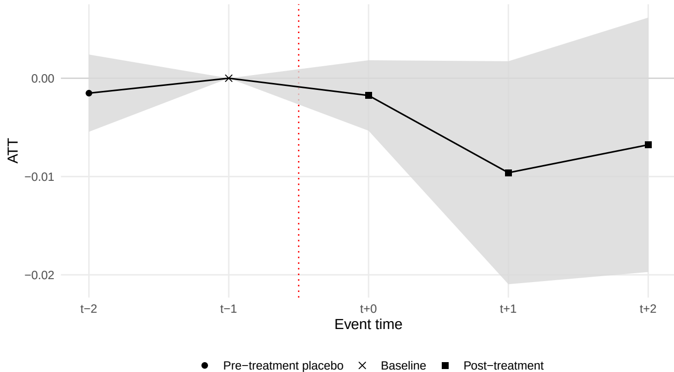
PanelMatch dynamic estimates – perc_plv_rinn (Mahalanobis – 3 neighbors)
