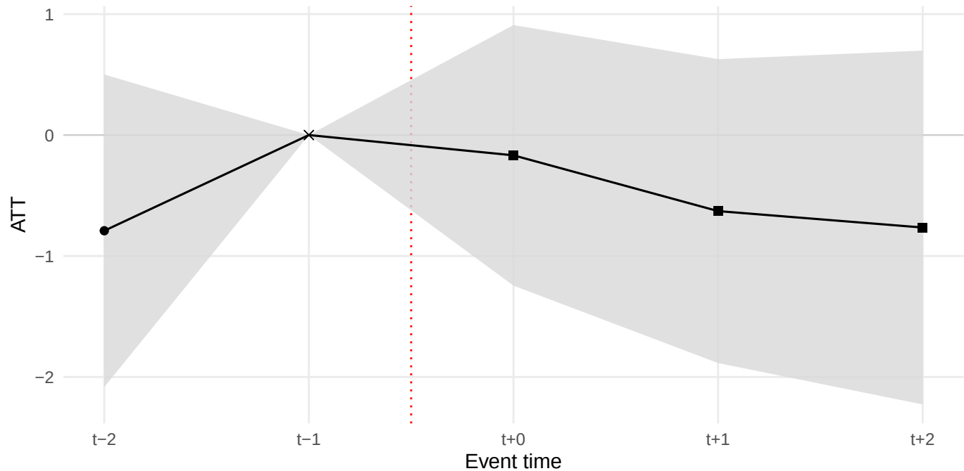
PanelMatch dynamic estimates – potenza_media (CBPS.weight)
