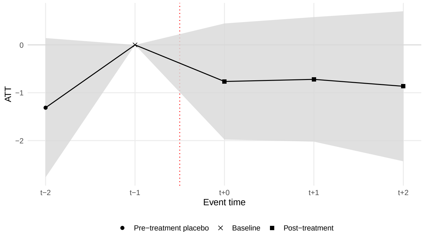
PanelMatch dynamic estimates – potenza_media (Mahalanobis – 3 neighbors)
