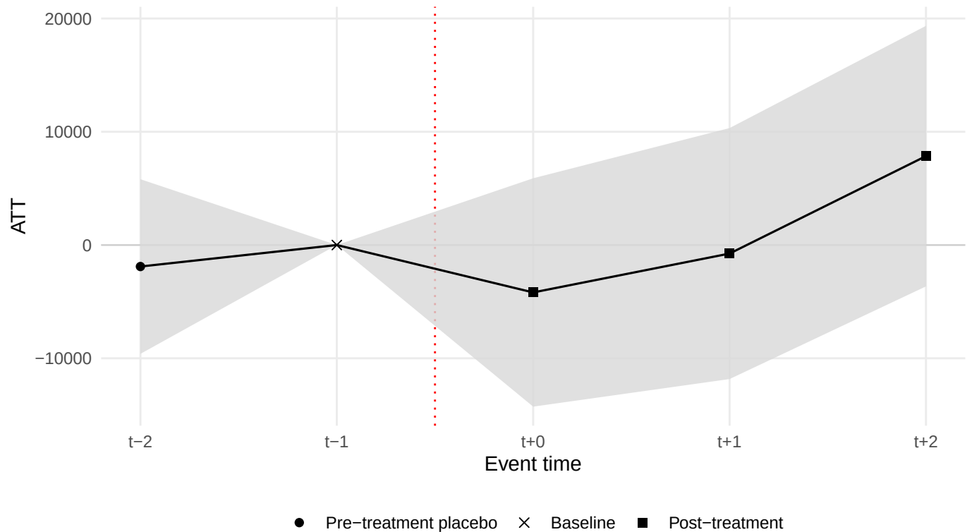
PanelMatch dynamic estimates – utile_perdita_esercizio (Mahalanobis – 3 neigh
