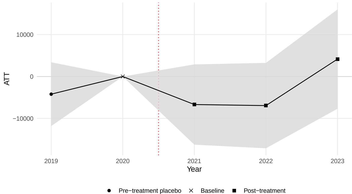
PanelMatch dynamic estimates – valore_aggiunto (CBPS.weight)
