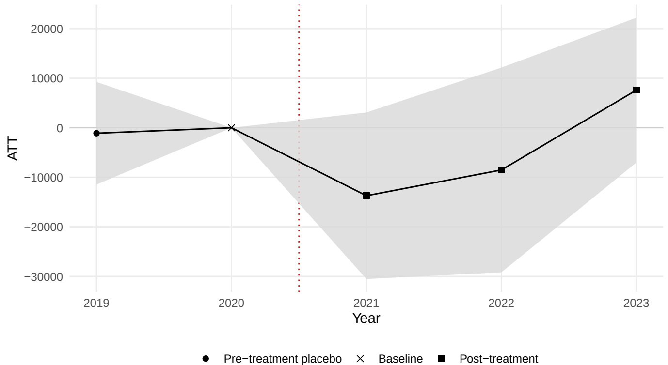
PanelMatch dynamic estimates – valore_aggiunto (Mahalanobis – 1 neighbor)
