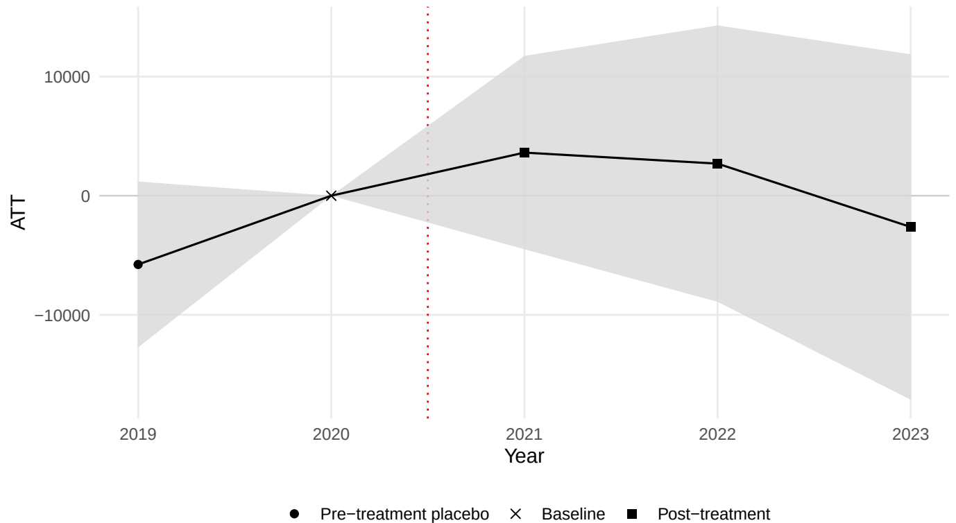
PanelMatch dynamic estimates – valore_nuovo (Mahalanobis – 1 neighbor)
