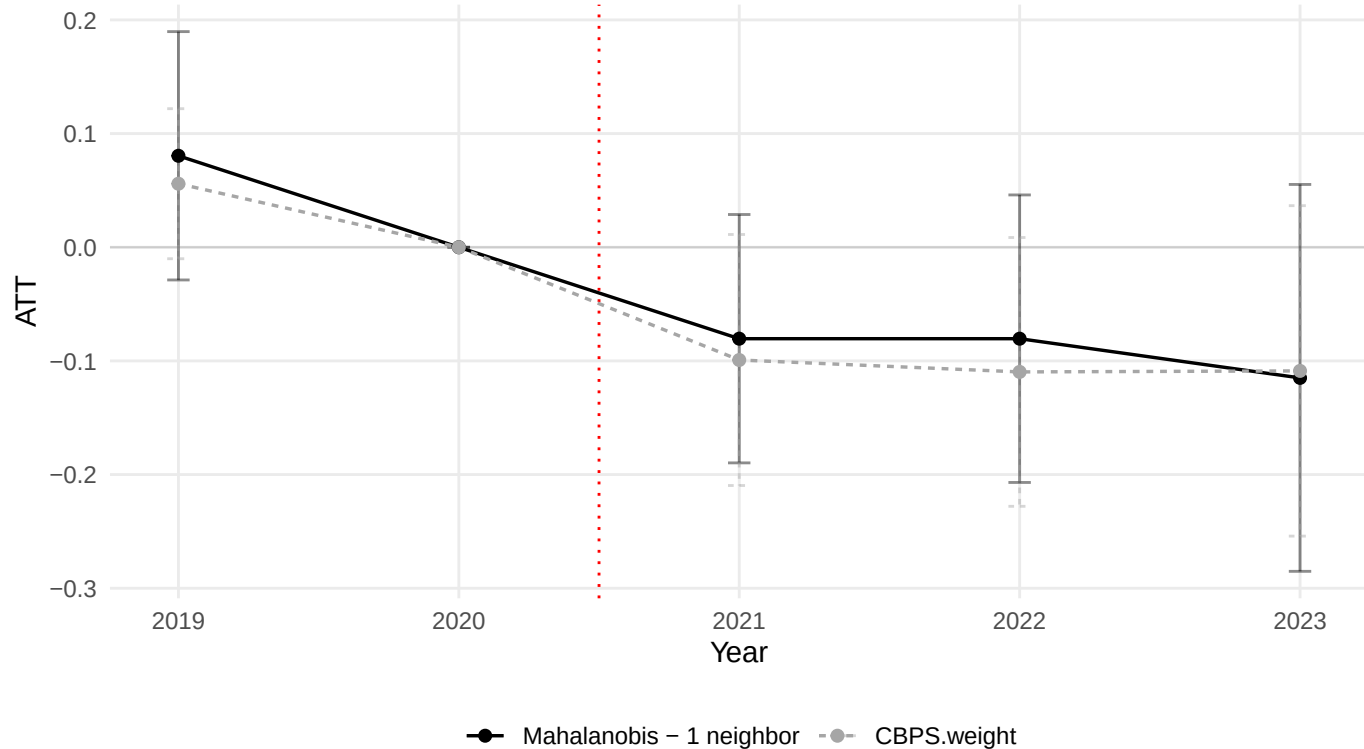
PanelMatch refinement comparison – assunto
