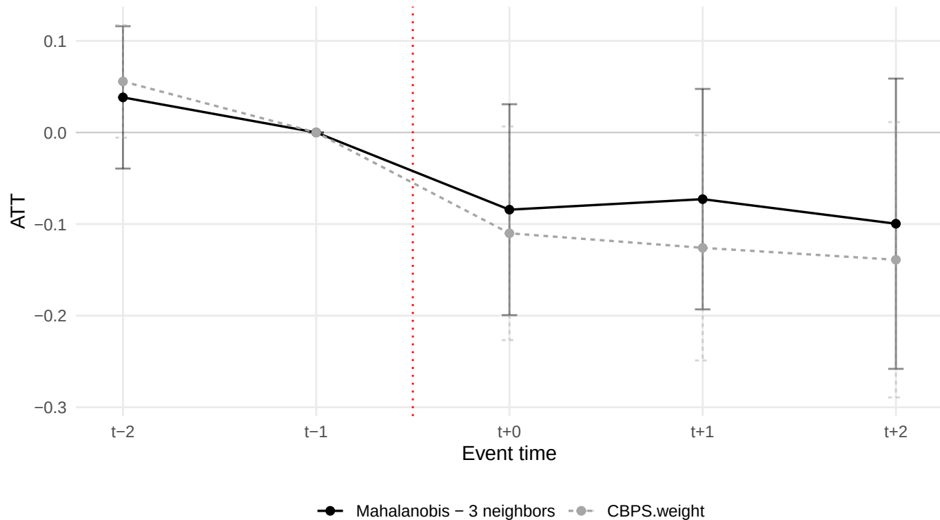
PanelMatch refinement comparison – n_manodopera
