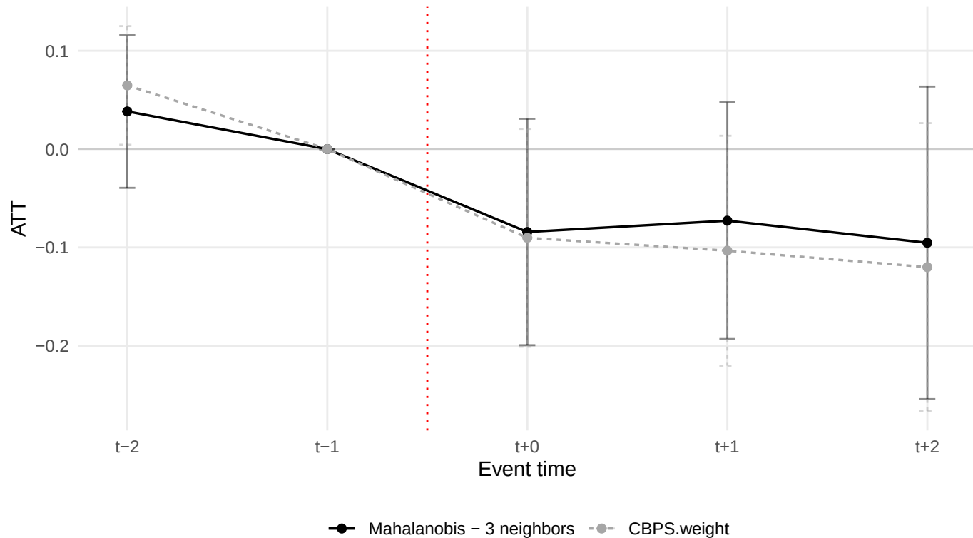
PanelMatch refinement comparison – n_manodopera_w
