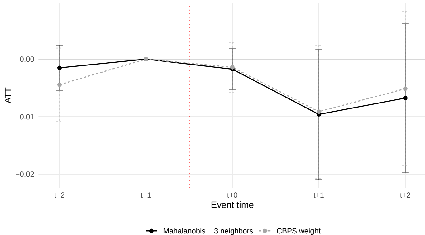
PanelMatch refinement comparison – perc_plv_rinn
