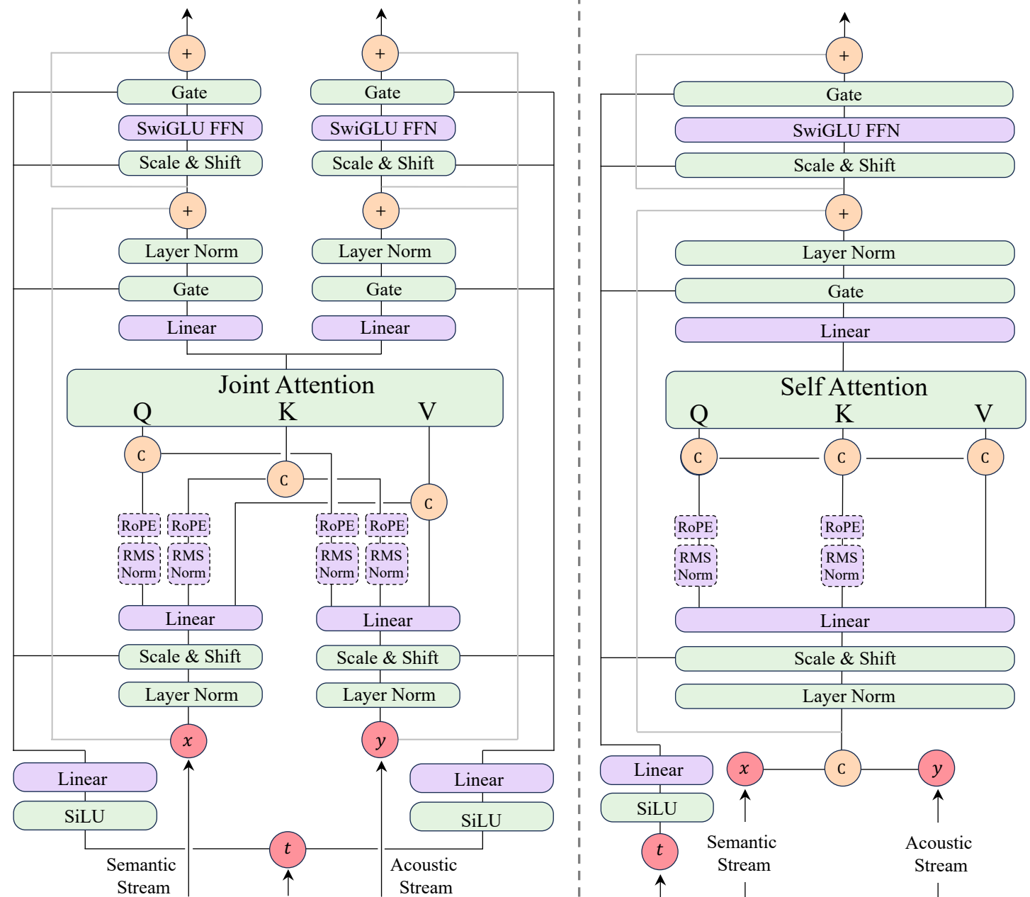
(b) Dual Stream MMDiT Block Architecture
