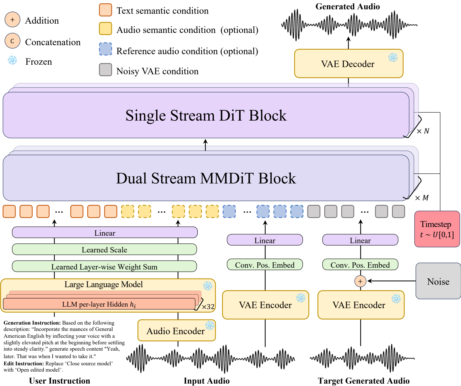
(a) AuK Model Architecture
