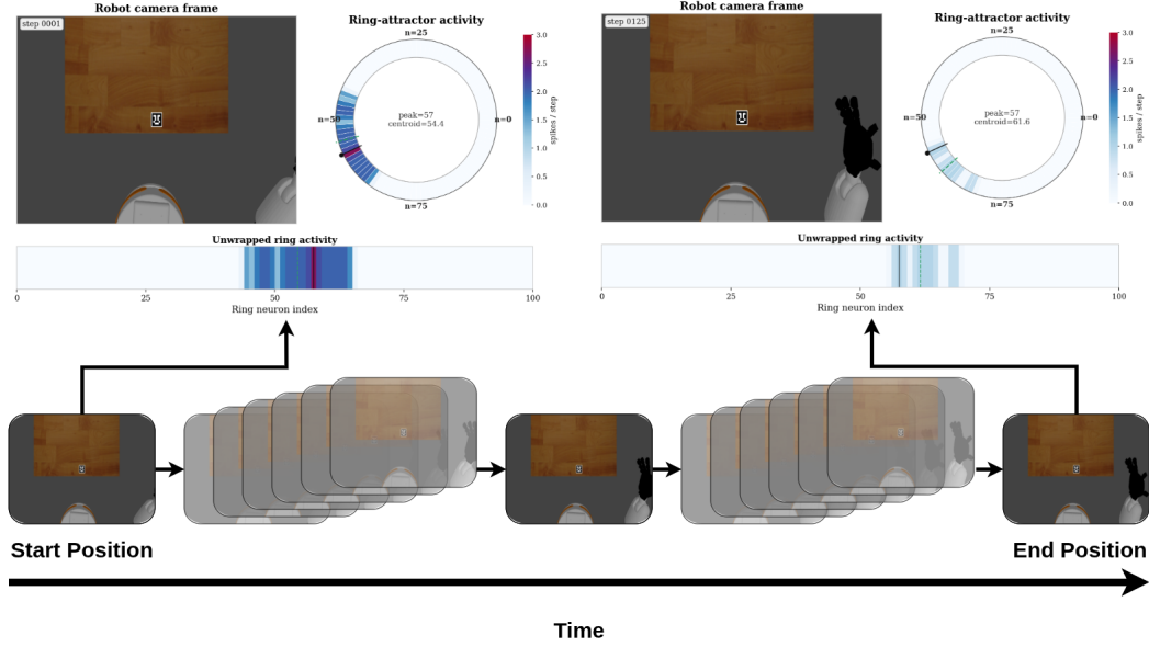
Figure 3: Robot-to-ring interface for the Tiago experiments. Each control step pairs a Tiago camera frame with the current spiking ring activity. The circular and unwrapped plots show the same population response, making the bump location and centroid visible during control. The timeline shows decoded gain-modulated commands moving the joint from start to target. Quantitative tracking results are reported in Figure 5, with additional analyses in Figures 7 and 8.
